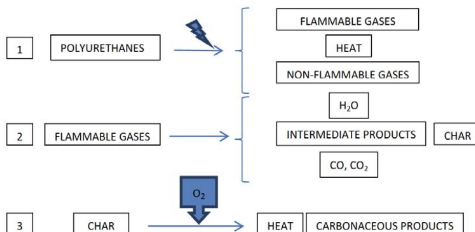
Figure 1: General mechanism of thermal decomposition of polyurethanes.
